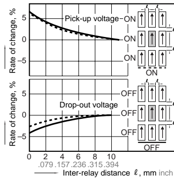
13-(3). Influence of adjacent mounting Tested sample: TXD2-12V, 6 pcs.
